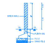
COMPOUND WALL DETAIL
