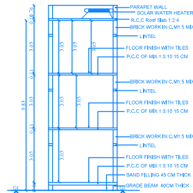
SECTION ON-AA
