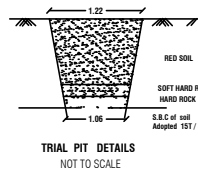
TRIAL PIT DETAILS NOT TO SCALE
