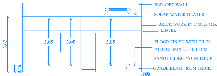
SECTION-AB
