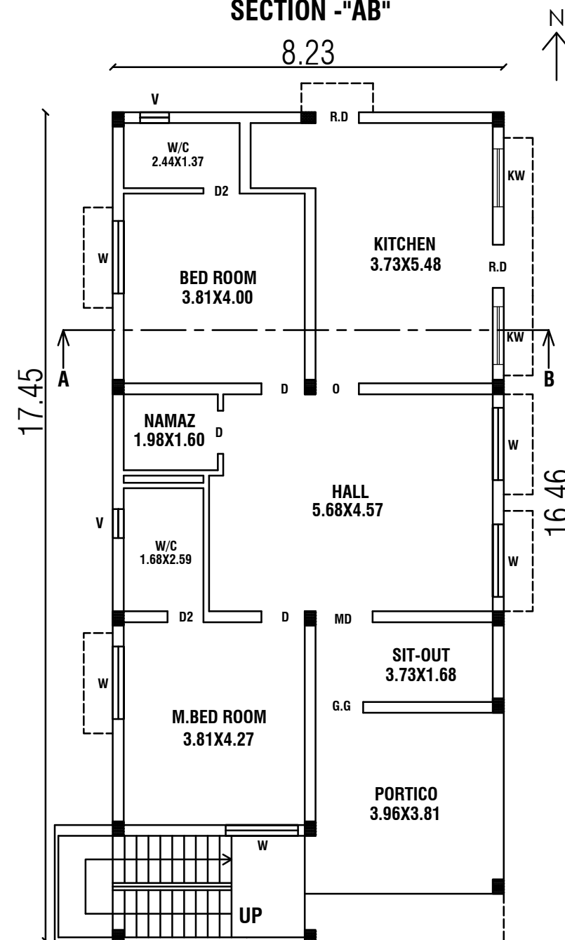
PRO.GROUND FLOOR PLAN
