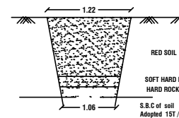
TRIAL PIT DETAILS NOT TO SCALE
