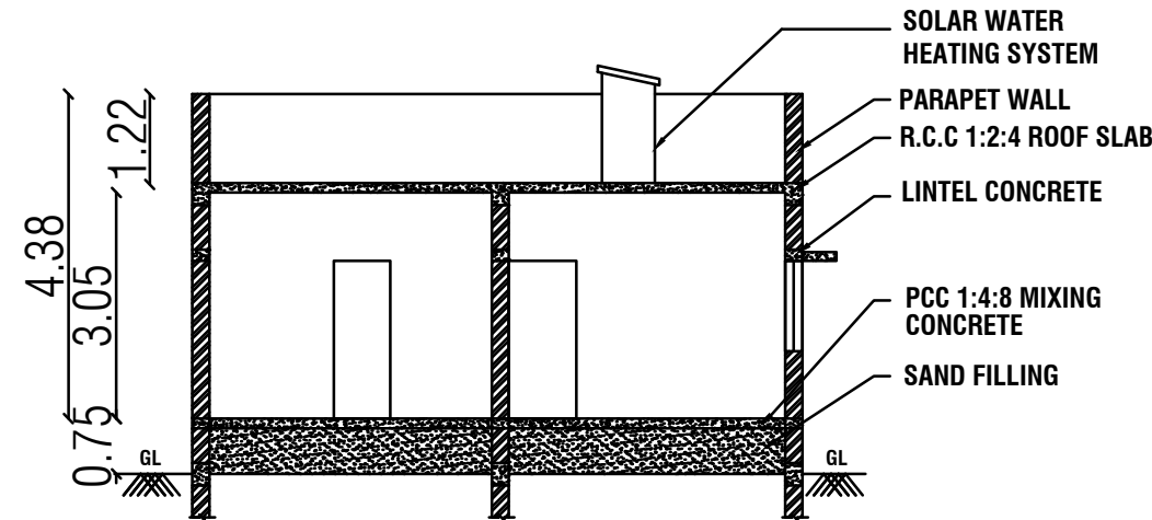
SECTION -"AB"
