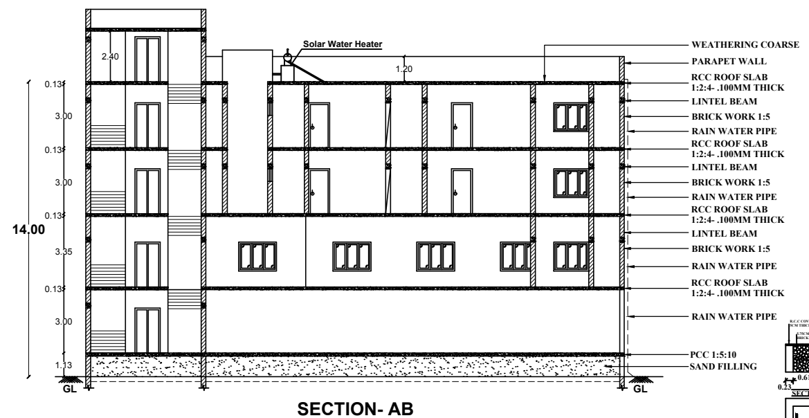
SECTION- AB
