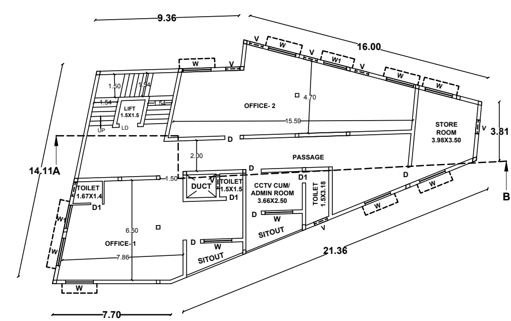
TYPICAL FLOOR PLAN SECOND & THIRD FLOOR PLAN
