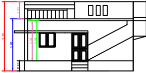
FRONT ELEVATION
