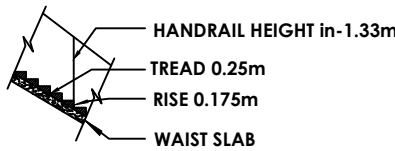
STAIRCASE DETAILS
