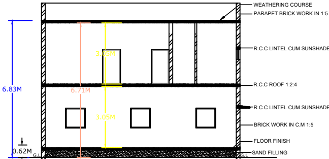
SECTION ON XX
