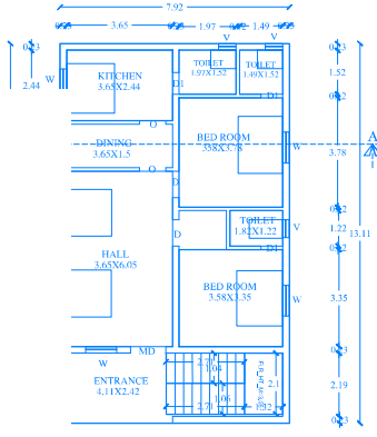
D. FIRST FLOOR PLAN
