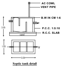
Septic tank detail
