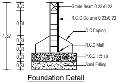
Foundation Detail
