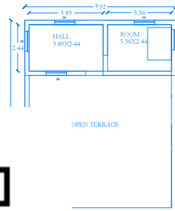
FLOOR PLAN
