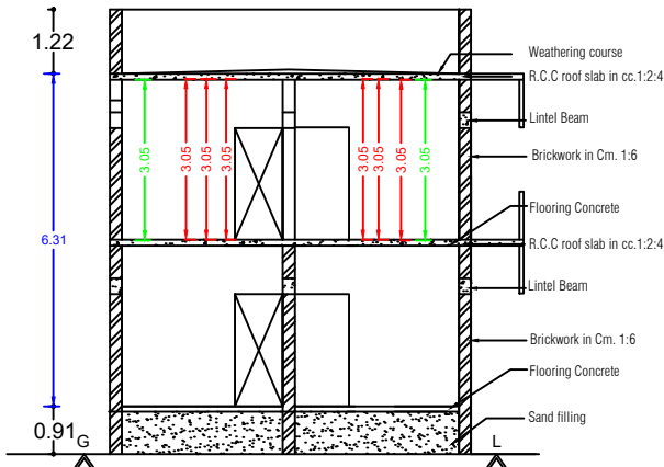
SECTION-AB
