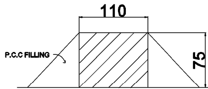
DWARF WALL SECTION NOT TO SCALE
