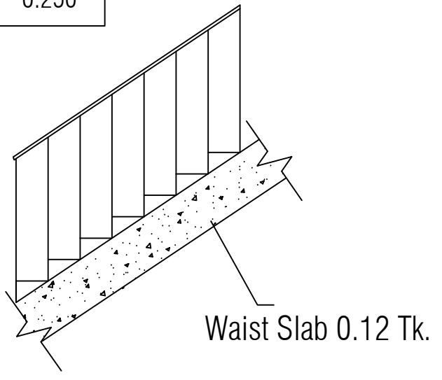
Staircase Details
