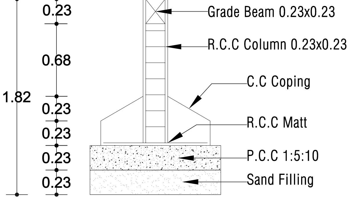
Foundation Detail
