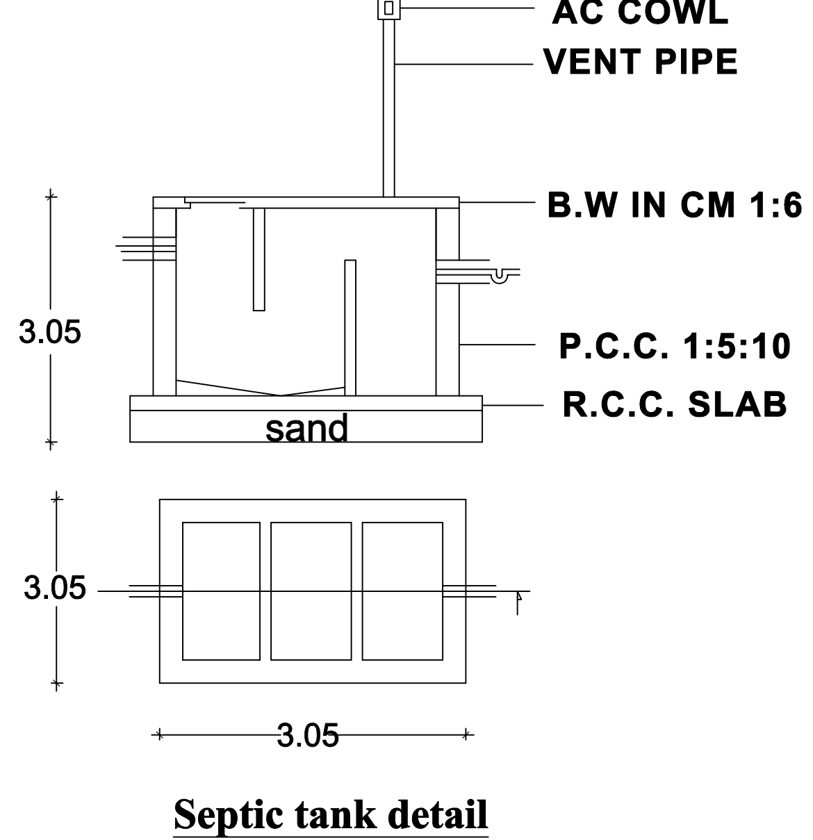
Septic tank detail
