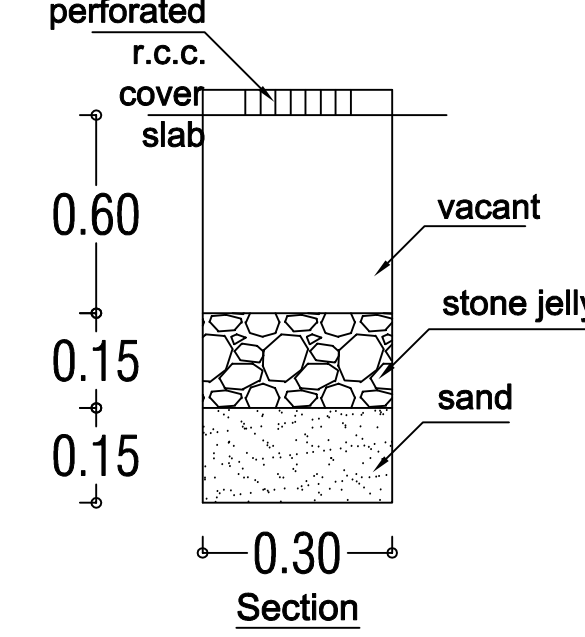
RAIN WATER PERCUSSION PIT
