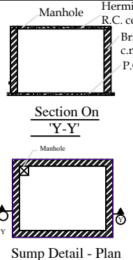
Sump Detail - Plan
