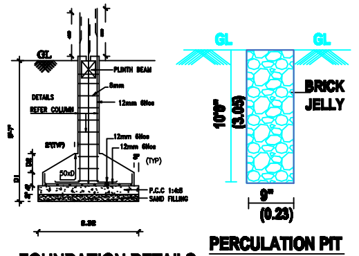
FOUNDATION DETAILS SCALE : 1:50.
