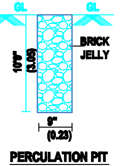
PERCOLATION PIT
