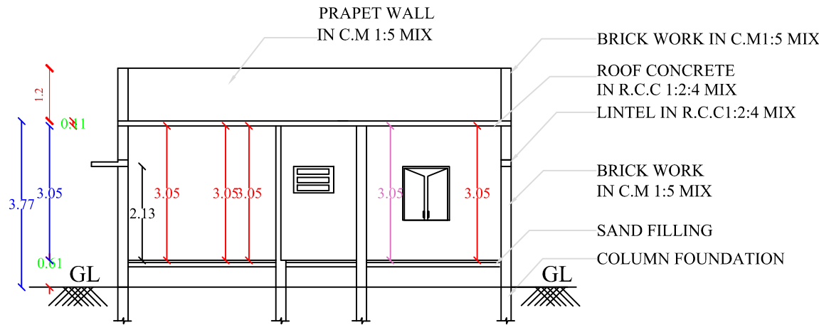
SECTION ON"XX"
