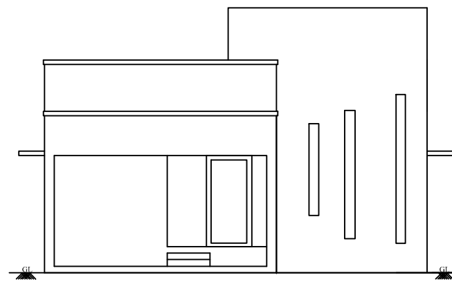
FRONT ELEVATION
