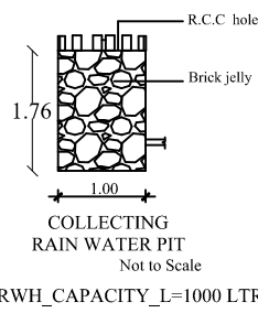
COLLECTING RAIN WATER PIT
