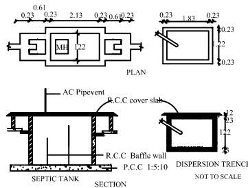
SEPTIC TANK
