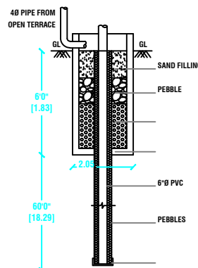
Section of Rain water Harvesting (from open terraced)
