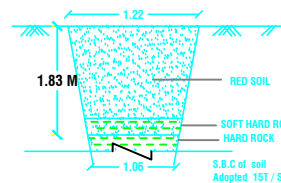
TRIAL PIT DETAILS
