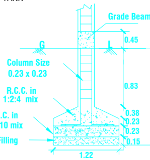
COLUMN DETAILS
