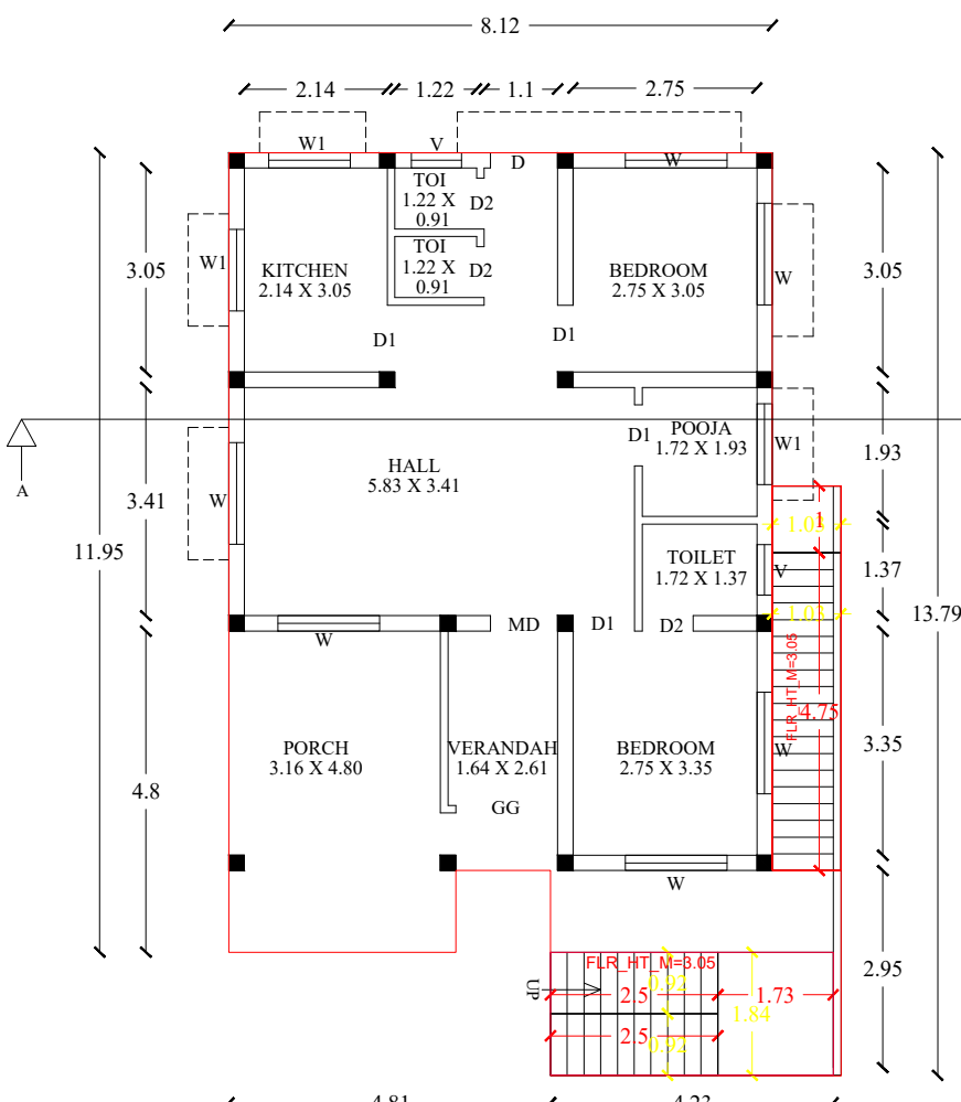
EXI.GROUND FLOOR PLAN
