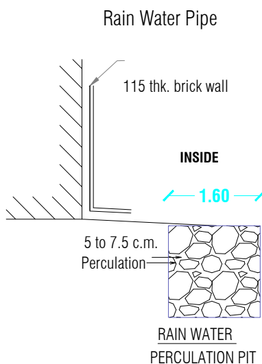
SECTION NO -"AA"
