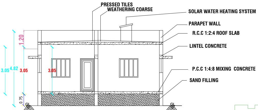
SECTION NO -"AA"
