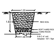
TRIAL PIT DETAILS NOT TO SCALE
