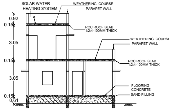
SECTION NP
