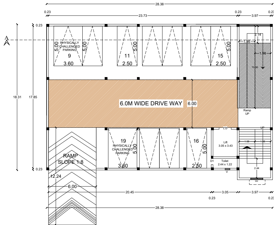
SEMI BASEMENT FLOOR PLAN
