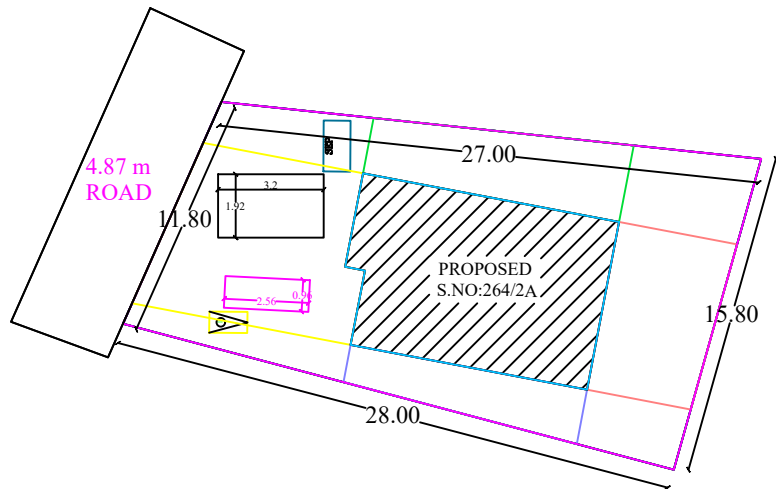
SITE PLAN
