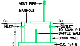
SECTION OF SEPTIC TANK
