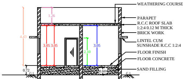
SECTION "N-R"
