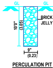
PERCOLATION PIT
