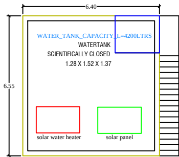
TERRACE FLOOR PLAN
