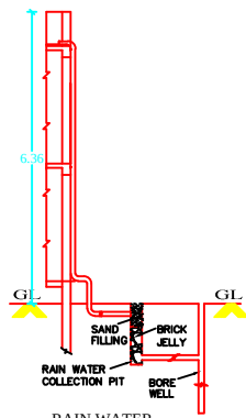
RAIN WATER HARVESTING SYSTEM RWHL_CAPACITY_L=1000LTRS
