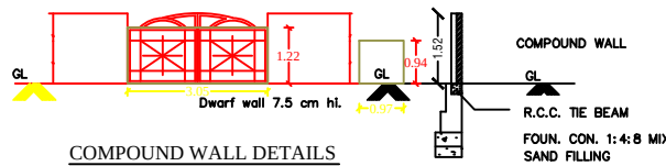
COMPOUND WALL DETAILS
