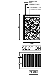
RAIN WATER HARVESTING PERCOLATION BED
