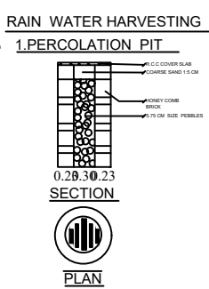
RAIN WATER HARVESTING 1. PERCOLATION PIT
