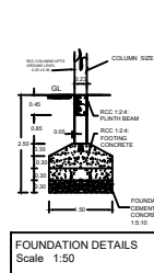
FOUNDATION DETAILS Scale: 1:50
