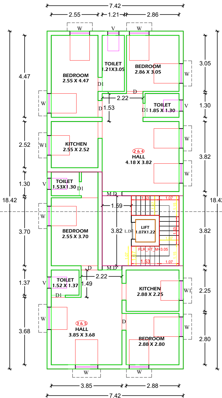
TYPICAL FIRST & SECOND FLOOR PLAN
