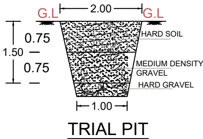
TRIAL PIT
