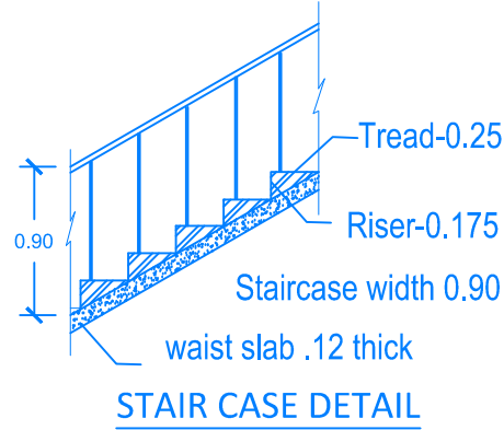
STAIR CASE DETAIL
