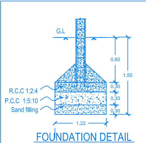
FOUNDATION DETAIL
