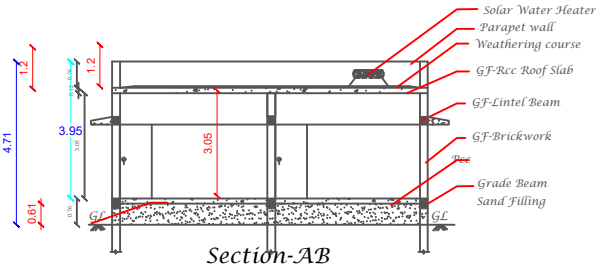
Section-AB
