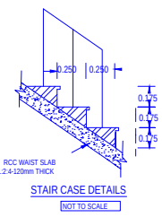
STAIR CASE DETAILS SCALE 1: 30
