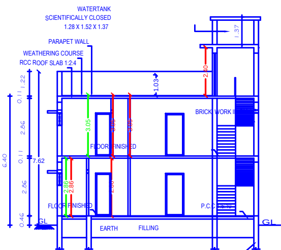
SECTION "A-B"
