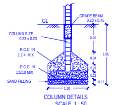
COLUMN DETAILS SCALE 1: 50
