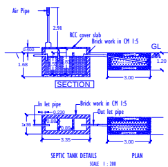
SEPTIC TANK DETAILS SCALE 1: 30
