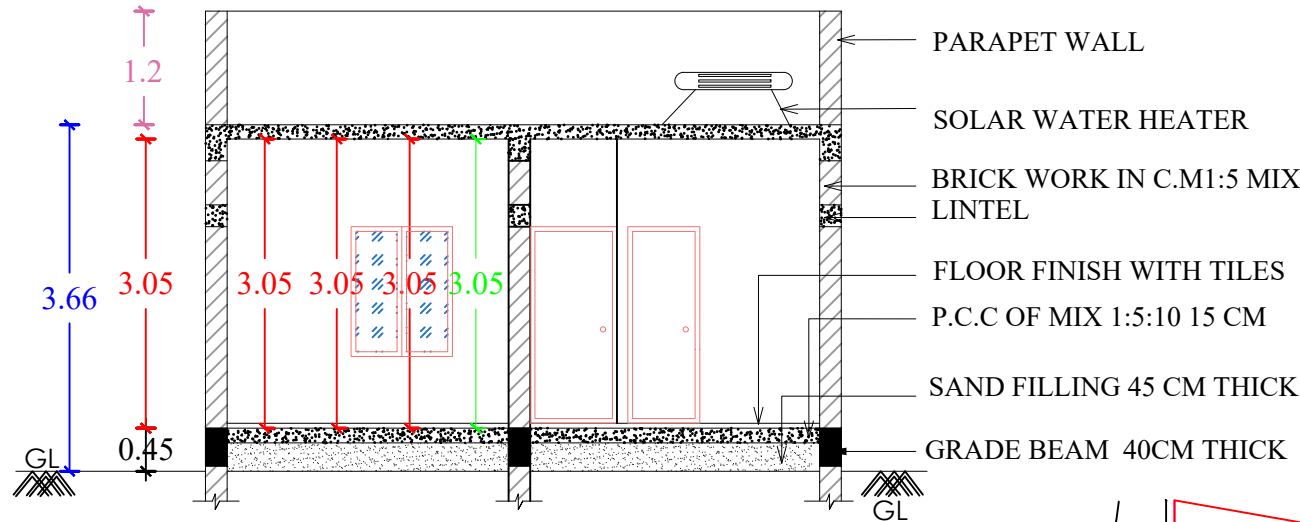
SECTION- AA1
