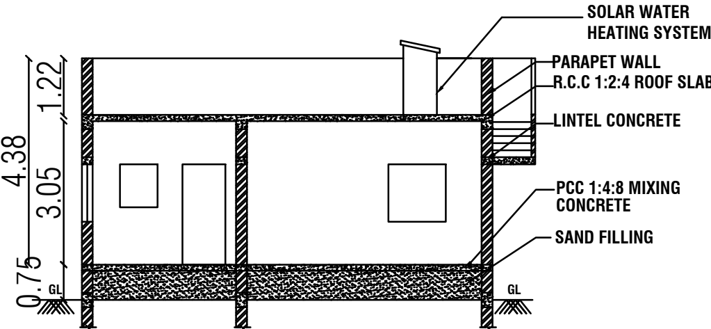
SECTION NO -"AB"
