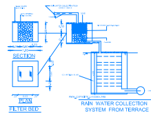
RAIN WATER COLLECTION SYSTEM FROM TERRACE
