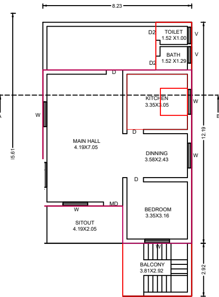
IRST FLOOR PLAN
