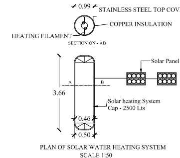
PLAN OF SOLAR WATER HEATING SYSTEM SCALE 1:50
