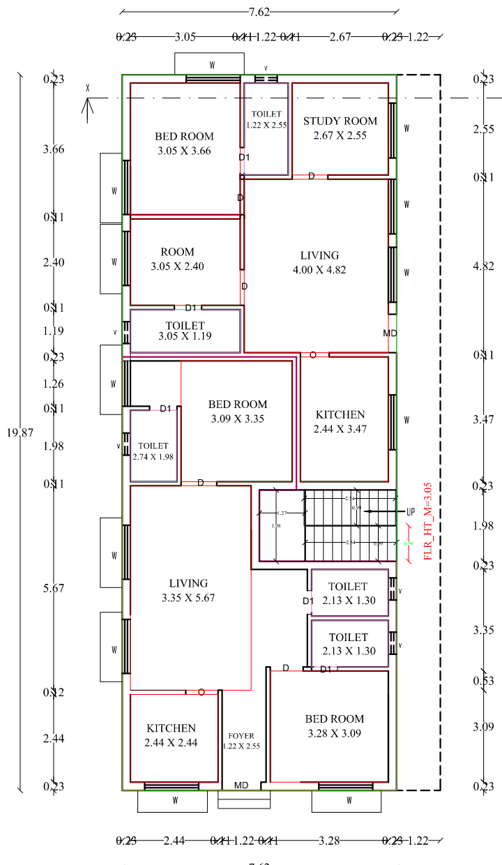
OR PLAN
