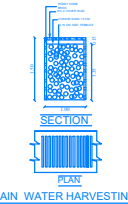
RAIN WATER HARVESTING PERCOLATION BED
