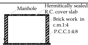
Section On 187 371
