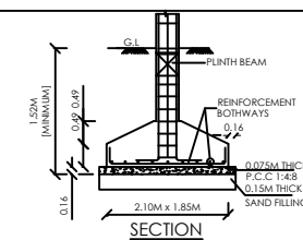
SECTION
