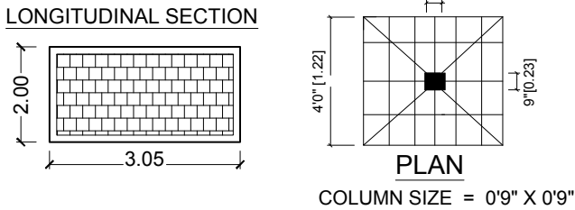
PLAN COLUMN SIZE = 0'9" X 0'9"
