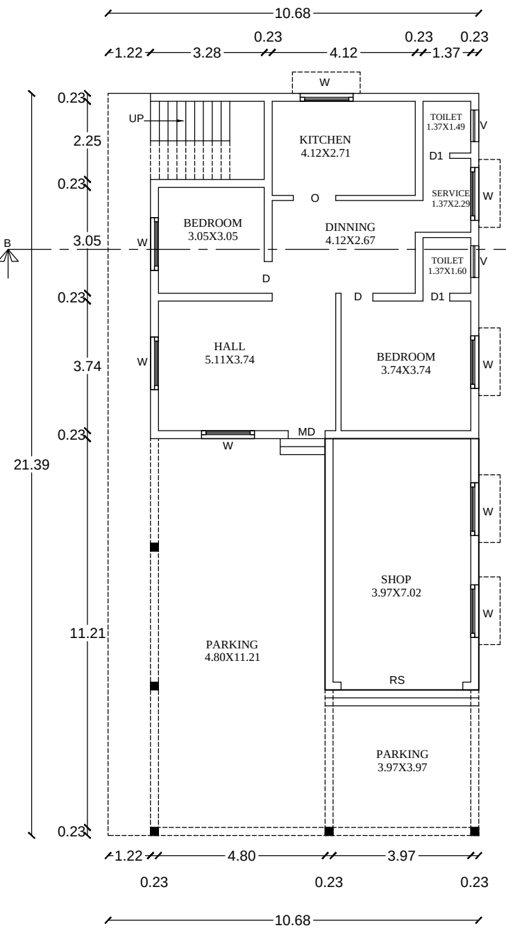
R PLAN
