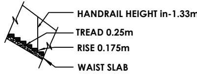
STAIRCASE DETAILS
