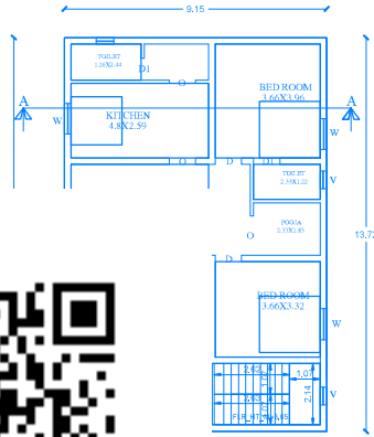
OR PLAN
