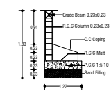
Foundation Details
