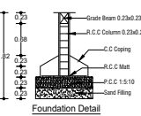
Foundation Detail
