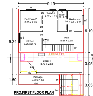
PRO.FIRST FLOOR PLAN
