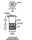
Foundation Detail
