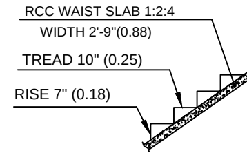
STAIRCASE DETAIL
