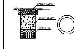
RAIN WATER HARVESTING SYSTEM
