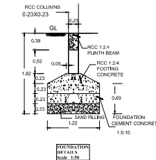
FOUNDATION DETAIL
