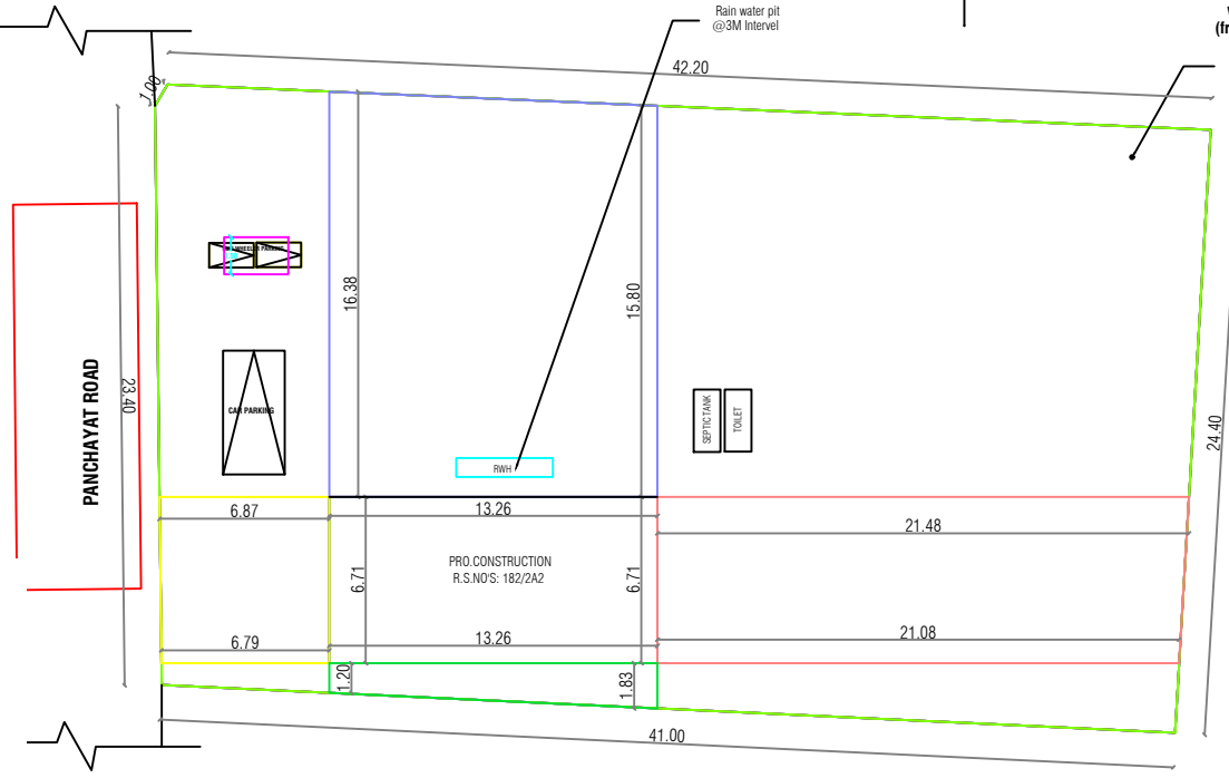
SITE PLAN
