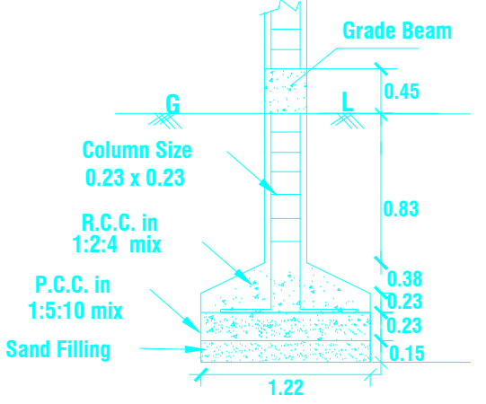
COLUMN DETAILS
