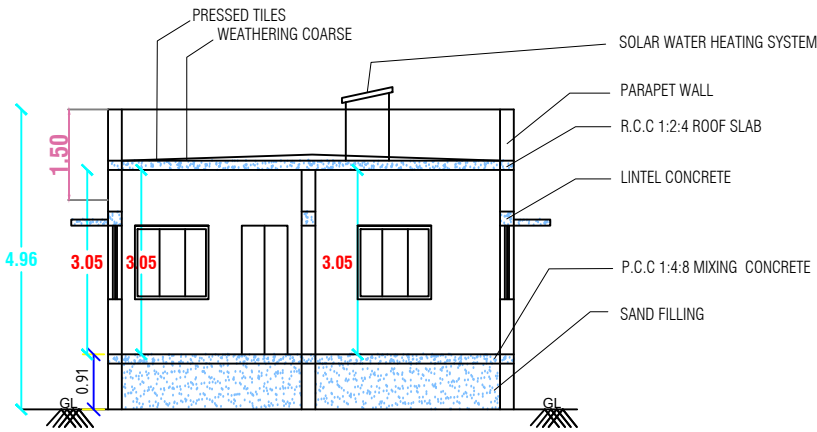
SECTION AT -"AA"
