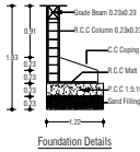
Foundation Details
