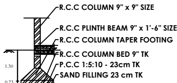
SECTION COLUMN DETAILS PLAN
