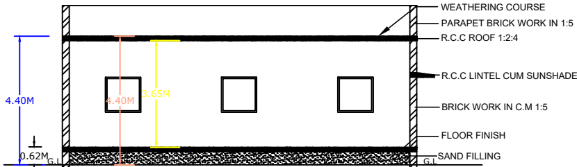
SECTION ON XX
