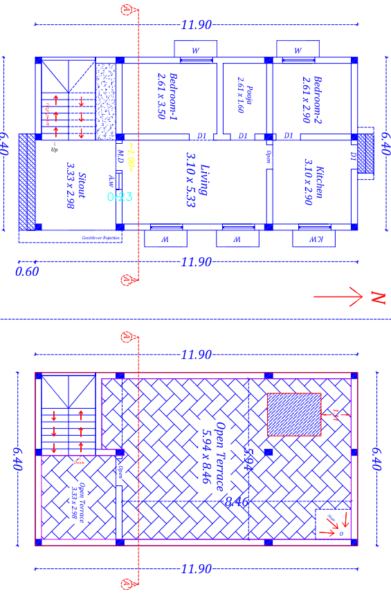
Proposal Ground Floor Residential Plan (Site Plan View is in South Facing)
