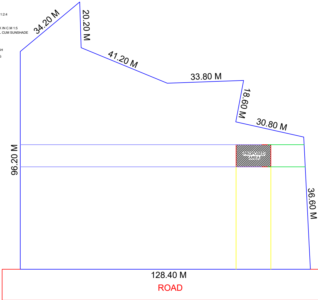
TOPO PLAN
