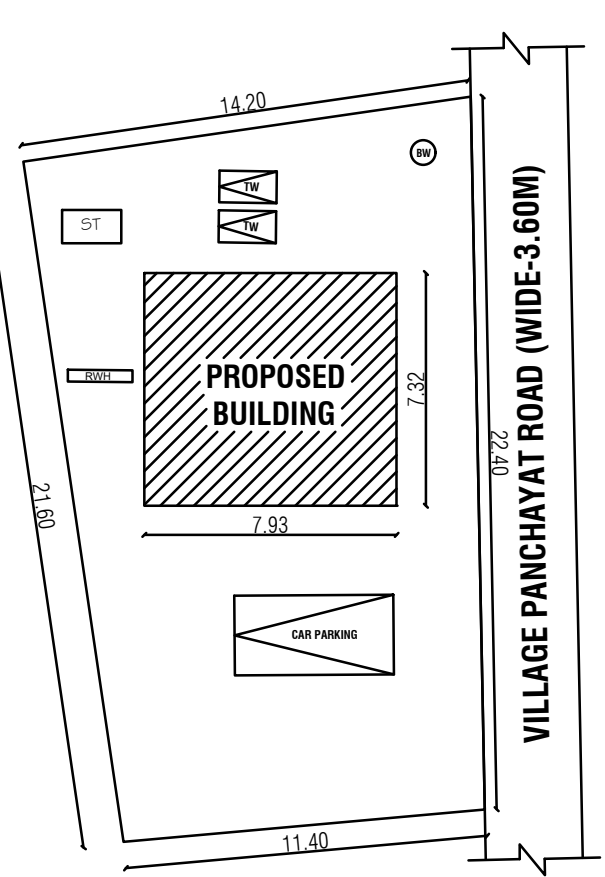
SOUTH SIDE MUTHUVEERAN & MUKILAN PROPERTY
