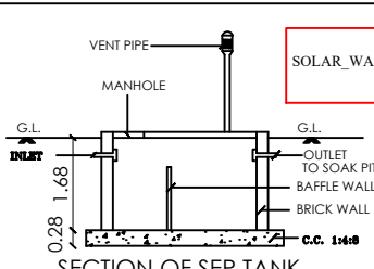
SECTION OF SEP.TANK
