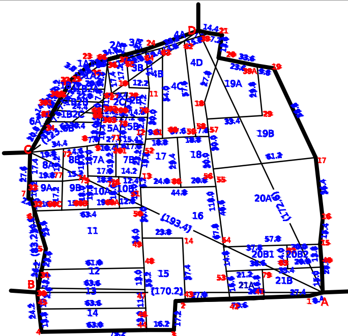
TOPO PLAN
