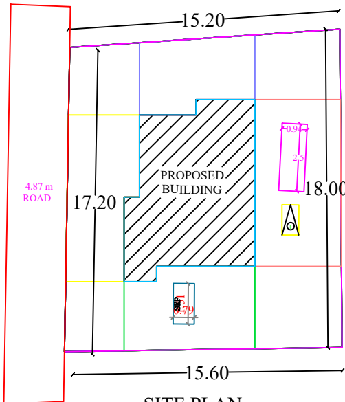
SITE PLAN
