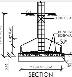
SECTION
